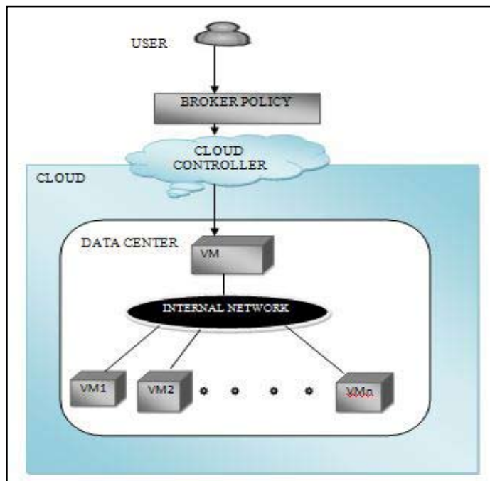
Figure 3: Architecture of a System Scheduling
