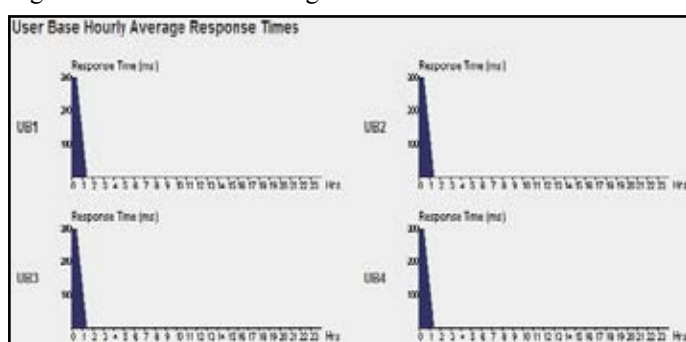
Figure 6: A Graph of User Base Hourly Average Response time Using RR Scheduler
