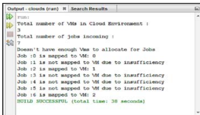
Figure 4: Random Resource Selection
