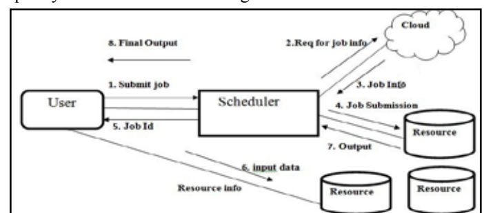
Figure 1 Scheduling in Cloud
